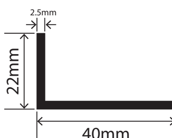
RCAP40X22L
