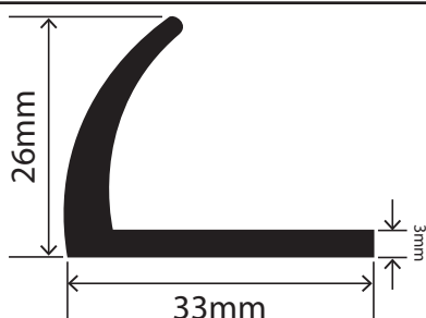
RCAP33X26W
