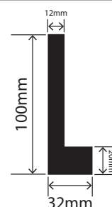
RCAP32X100W
